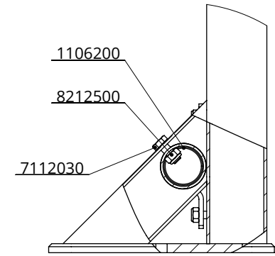
detail C (1 : 5)
